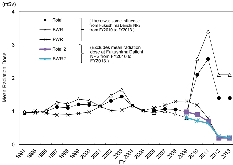
Trends in Mean Radiation Dose in Commercial Nuclear Power Reactors and Fukushima Daiichi NPS (1F) by Fiscal Year
