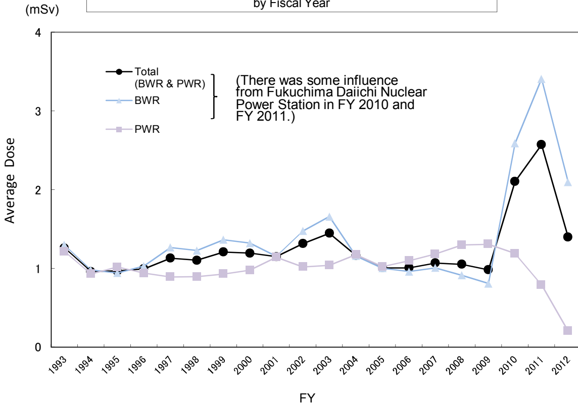
Trends of Average Radiation Dose at Commercial Nuclear Power Reactors by Fiscal Year
