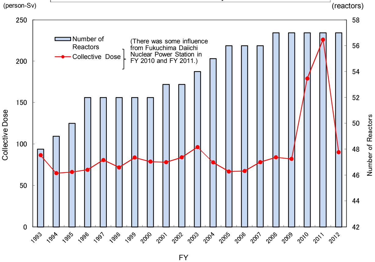
Trends of Collective Radiation Dose at Commercial Nuclear Power Reactors and the Number of Reactors by Fiscal Year
