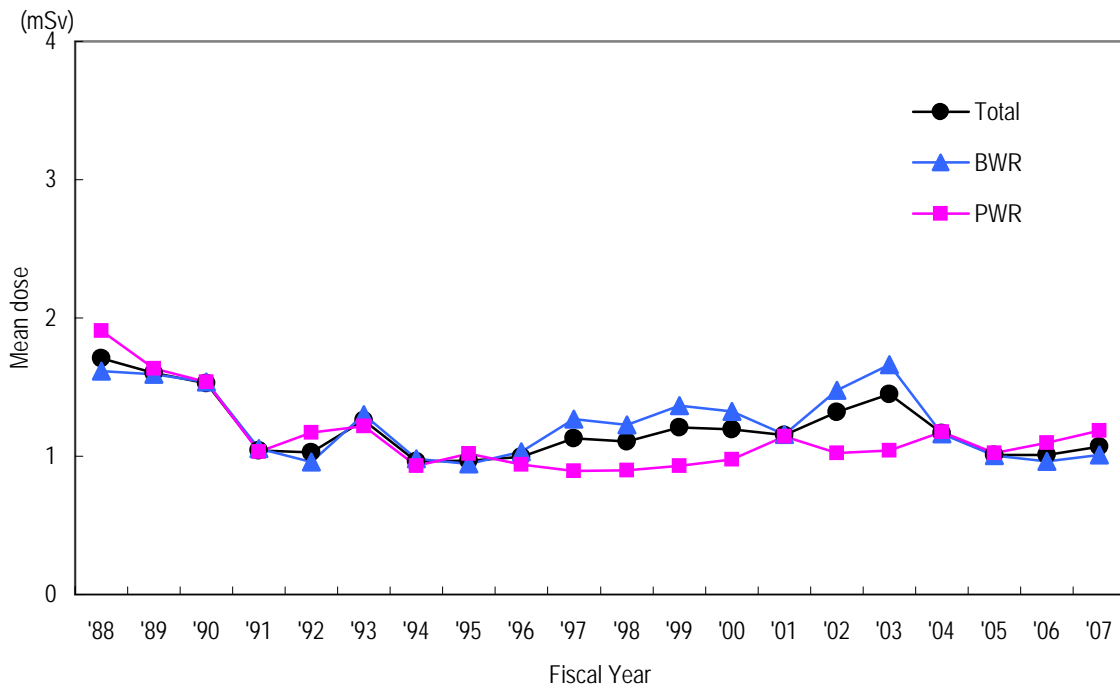
Trends in Average Individual Dosages at Commercial Power Reactor Facilities by Fiscal Year
