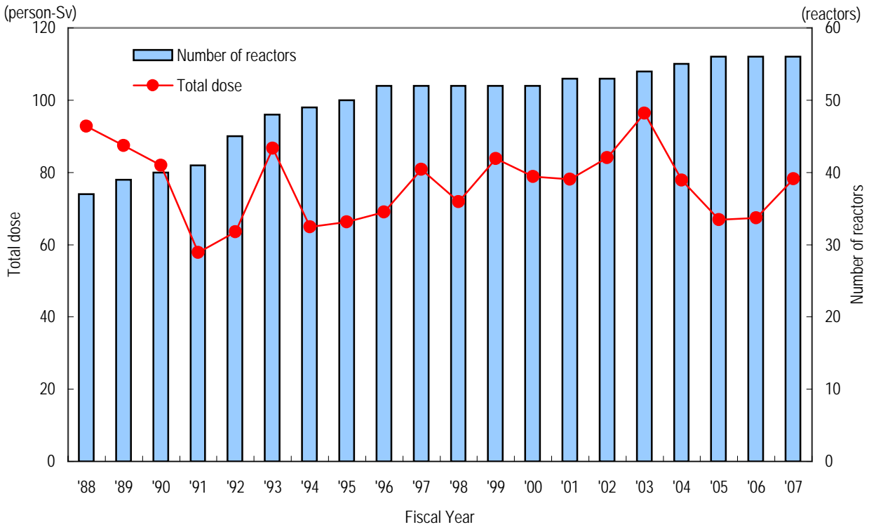
Trends in Collective Dosages at Commercial Power Reactor Facilities and the Number of Reactors by Fiscal Year
